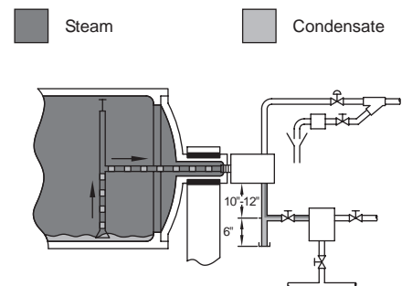
Figure CG-22-5. Large cylinder, syphon drained. 300 kg/h from a 1 200 mm diameter, 2 500 mm long cylinder dryer with 2,8 m 3 of space at 2 barg. The safety factor is 3:1 with a DC and 8:1 with an IB.
