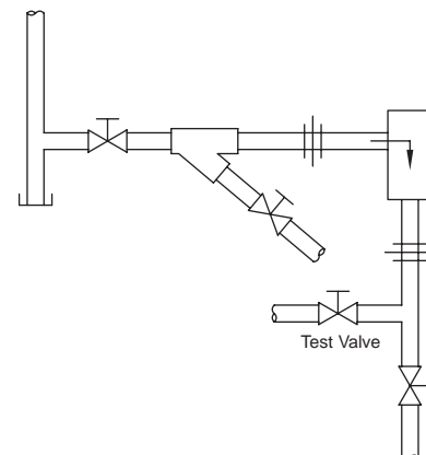
Figure CG-55-3. Typical Thermostatic Hookup
