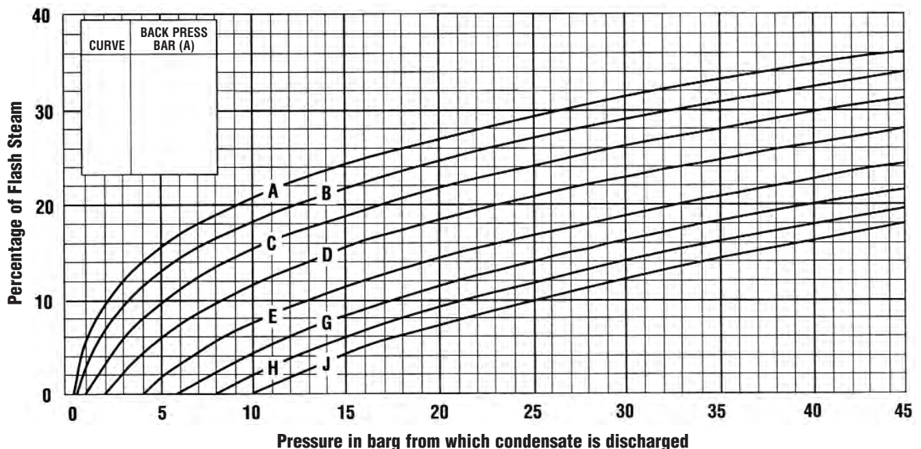
Chart CG-11-1. Percentage of flash steam formed when discharging condensate to reduced pressure.
