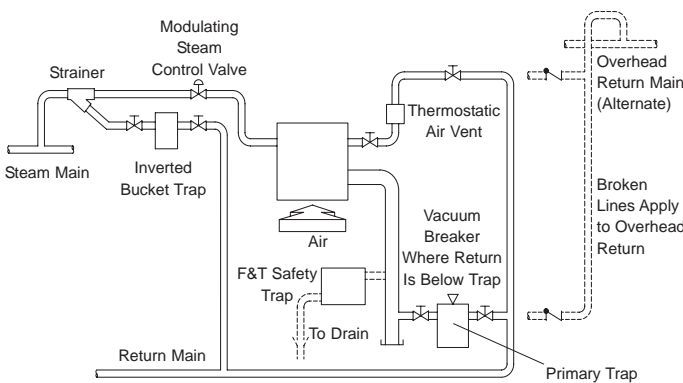
Figure CG-33-2. Trapping and Venting Air Heat Coil
