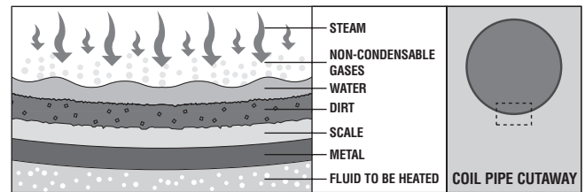
Figure CG-13-1. Potential barriers to heat transfer: steam heat and temperature must penetrate these potential barriers to do their work.
