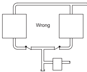
Figure CG-22-1. Two steam-consuming units drained by a single trap, referred to as group trapping, may result in short circuiting.
