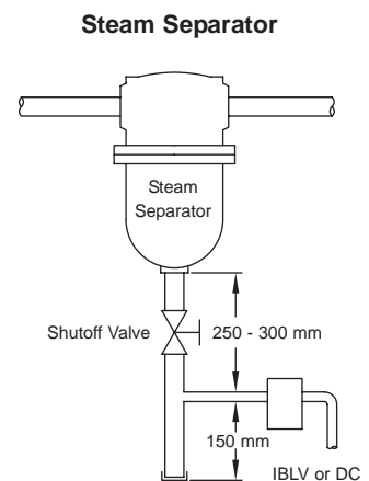
Figure CG-27-4. Drain downstream side of separator. Full-size drip leg and dirt pocket are required to ensure positive and fast flow of condensate to the trap.
