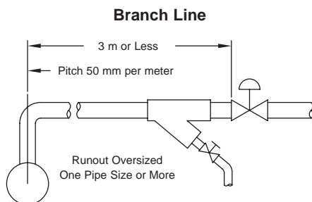
Figure CG-27-1. Piping for runout less than 3 m. No trap required unless pitch back to supply header is less than 50 mm per meter.
