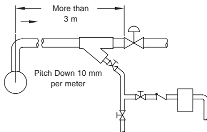
Figure CG-27-2. Piping for runout greater than 3 m. Drip leg and trap required ahead of control valve. Strainer ahead of control valve can serve as drip leg if blowdown connection runs to an inverted bucket trap. This will also minimize the strainer cleaning problem. Trap should be equipped with an internal check valve or a swing check installed ahead of the trap.
