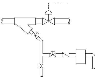
Figure CG-26-1. Trap draining strainer ahead of PRV.
