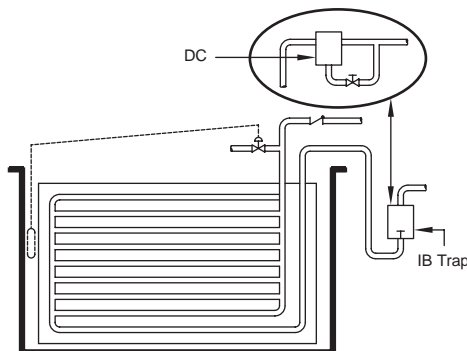
Figure CG-37-1. Thermostatic Controlled Embossed Coil, Syphon Drained
