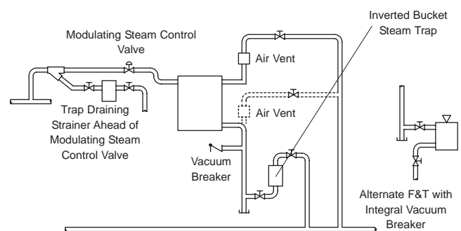
Figure CG-35-1. Process Air Heater
