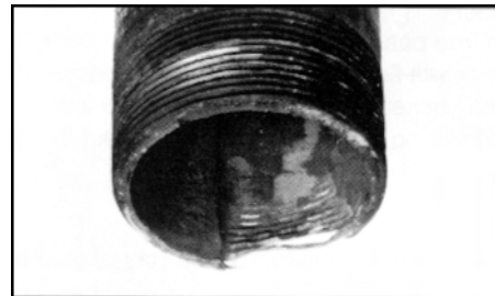
Figure CG-15-2. CO 2 gas combines with condensate allowed to cool below steam temperature to form carbonic acid, which corrodes pipes and heat transfer units. Note groove eaten away in the pipe illustrated.
