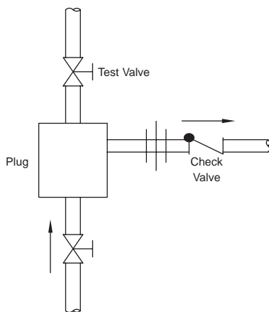
Figure CG-53-3. Typical IB By-pass Hookup
