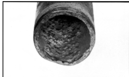
Figure CG-15-3. Oxygen in the system speeds corrosion (oxidation) of pipes, causing pitting such as shown here.
