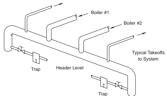
Figure CG-24-2. Boiler Headers
