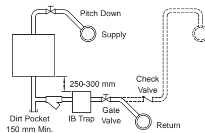
Figure CG-33-4. Generally approved method of piping and trapping low-pressure (under 1 barg) vertical discharge heaters.
