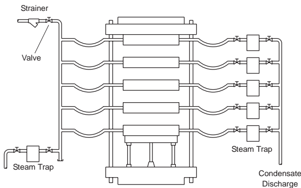
Figure CG-44-1. Product Confined In Steam Jacketed Press
