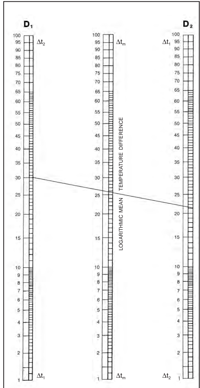
Chart CG-41-1. Mean Temperature Difference Chart for Heat Exchange Equipment
