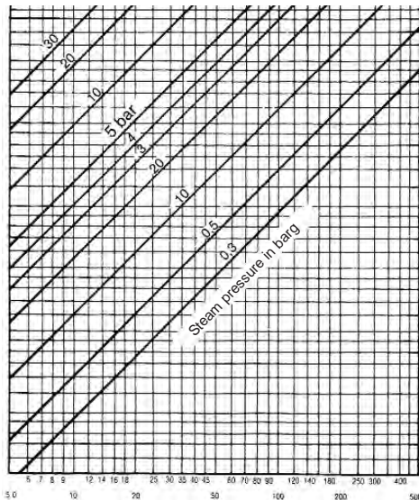
Chart CG-59-1. Pressure Drop in Saturated Steam Lines
