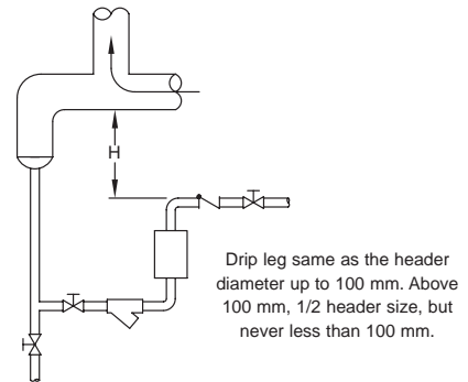
Figure CG-26-3. Trap draining drip leg at riser. Distance "H" in meters divided by 10 = static head pressure (bar) for forcing water through the trap.
