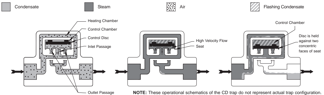
Figure CG-19-1. Operation of Controlled Disc Traps
