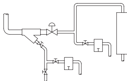
Figure CG-27-3. Regardless of the length of the runout, a drip leg and trap are required ahead of the control valve located below steam supply. If coil is above control valve, a trap should also be installed at downstream side of control valve.
