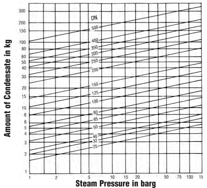
Chart CG-25-1. Amount of Condensate for 20 m of Pipe Heated From 0°C to Saturated Steam Temperature
