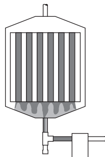
Figure CG-22-4. Multiple pipes, modulated pressure gravity flow to trap. 300 kg/h of condensate from unit heater at 5 barg. Multiple tubes create minor short-circuiting hazard. Use 3:1 safety factor at 2,5 barg.
