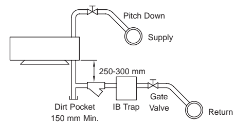
Figure CG-33-4. Generally approved method of piping and trapping low-pressure (under 1 barg) vertical discharge heaters.
