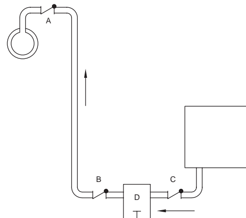
Figure CG-53-4. Typical IB By-pass Hookup, Bottom Inlet – Top Outlet
