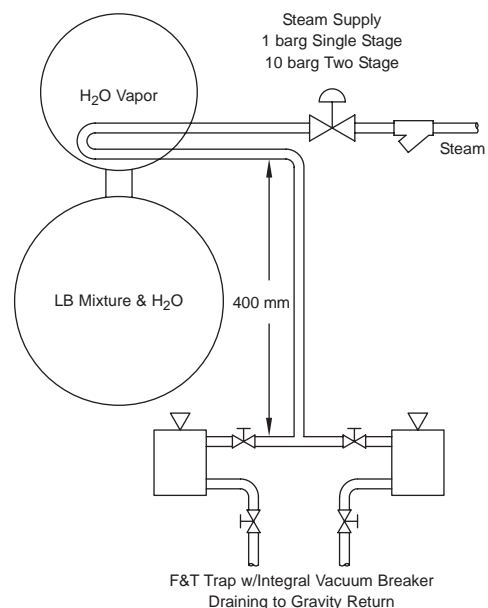
Figure CG-50-1. Generally approved method of piping steam absorption machine with standby trapping system.
