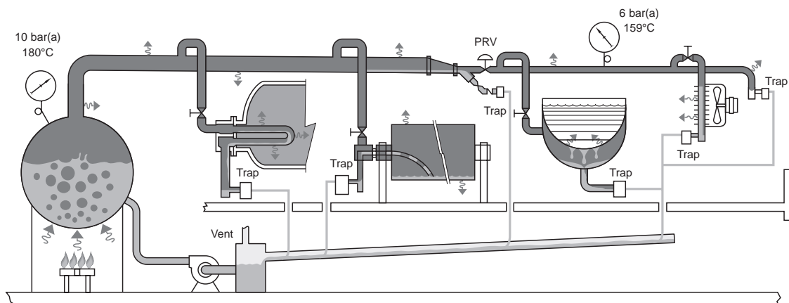
Figure CG-13-4. Note that heat radiation from the distribution system causes condensate to form and, therefore, requires steam traps at natural low points or ahead of control valves. In the heat exchangers, traps perform the vital function of removing the condensate before it becomes a barrier to heat transfer. Hot condensate is returned through the traps to the boiler for reuse.
