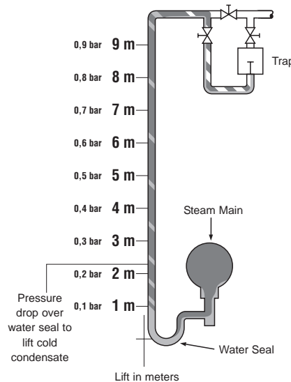
Figure CG-23-2. Condensate from gravity drain point is lifted to trap by a syphon. Every 1 m of lift reduces pressure differential by 0,1 bar. Note seal at low point and the trap's internal check valve to prevent backflow.
