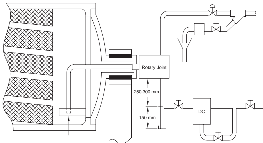
Figure CG-47-1. Product Inside Dryer
