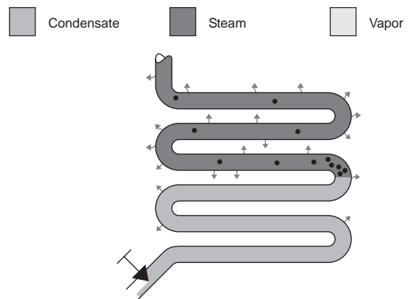
Figure CG-13-3. Coil half full of condensate can't work at full capacity.
