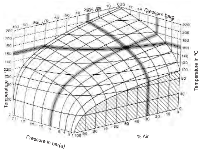
Chart CG-14-1. Air Steam Mixture
