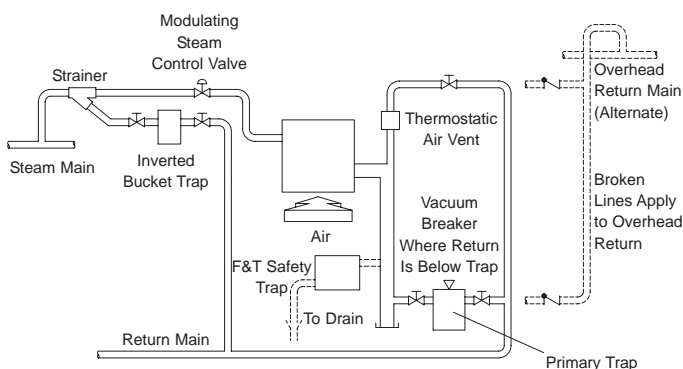
Figure CG-33-4. Generally approved method of piping and trapping low-pressure (under 1 barg) vertical discharge heaters.
