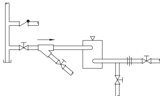
Figure CG-54-3. Typical F&T Hookup
