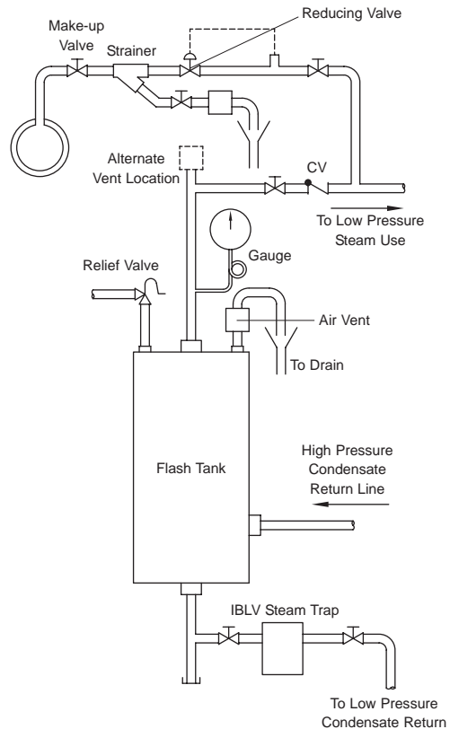
Figure CG-48-1. Typical Flash Tank Piping Sketch
