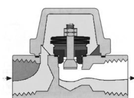
Figure CG-19-2. Operation of Bimetallic Steam Traps
