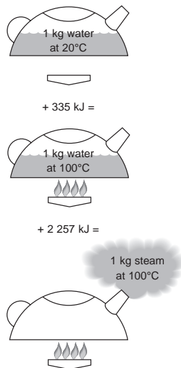
Figure CG-12-1. These drawings show how much heat is required to generate one kg of steam at atmospheric pressure. Note that it takes 4,186 kJ for every 1°C increase in temperature up to the boiling point, but that it takes much more kJ to change water at 100°C to steam at 100°C.
