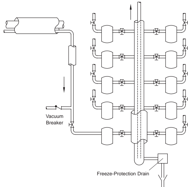
Typical Tracer Installation
