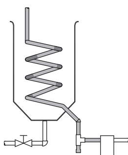
Figure CG-22-3. Continuous coil, constant pressure gravity flow to trap. 300 kg/h of condensate from a single copper coil at 3 barg. Gravity drainage to trap. Volume of steam space very small. 2:1 safety factor.
