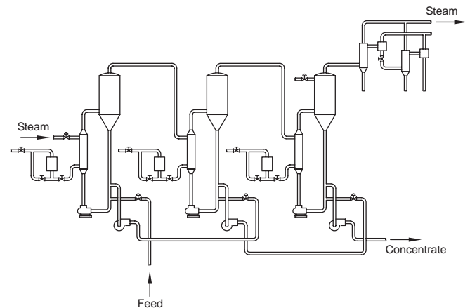
Figure CG-39-2. Triple Effect Evaporator System
