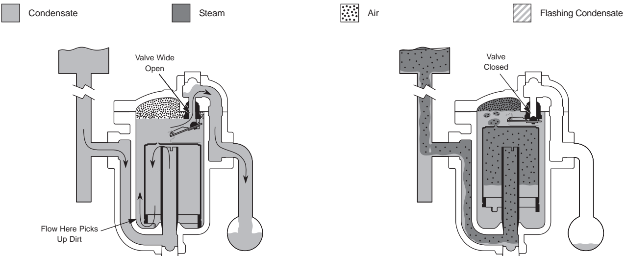
Figure CG-16-1. Operation of Inverted Bucket Steam Trap (at pressures close to maximum)
