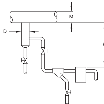
Figure CG-26-2. Trap draining drip leg on main.
