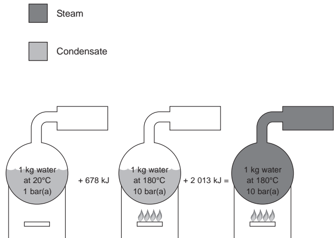
Figure CG-12-2. These drawings show how much heat is required to generate one kg of steam at 10 bar(a) pressure. Note the extra heat and higher temperature required to make water boil at 10 bar(a) pressure than at atmospheric pressure. Note, too, the lesser amount of heat required to change water to steam at the higher temperature.
