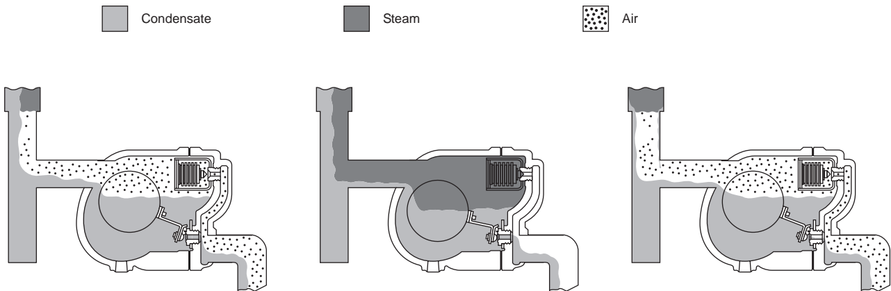
Figure CG-18-1. Operation of F&T Steam Trap
