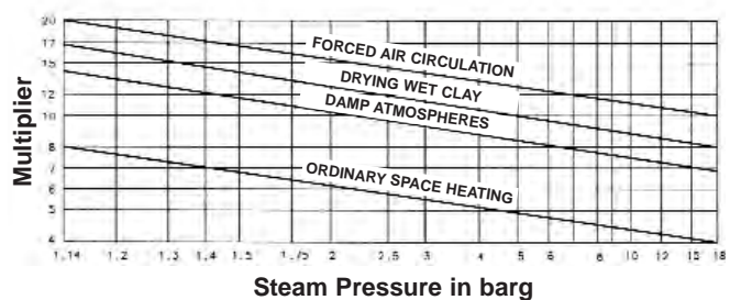
Chart CG-32-1. Multipliers for Sizing Traps for Multiple Coils
