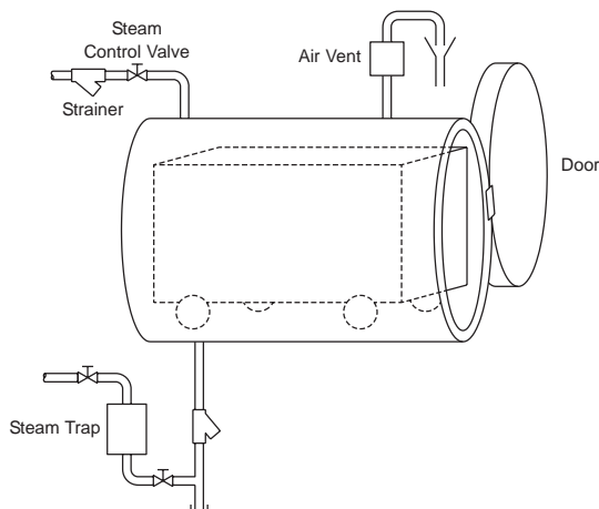
Figure CG-45-1. Direct Steam Injection Into Product Chamber
