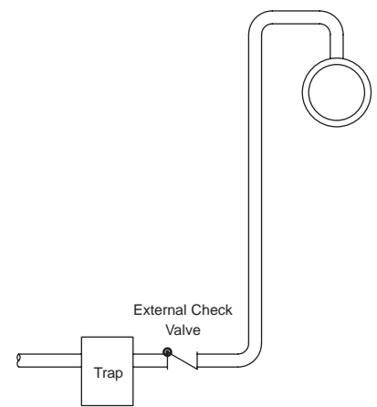
Figure CG-23-3. When trap valve opens, steam pressure will elevate condensate. Every 1 m of lift reduces pressure differential by 0,1 bar.
