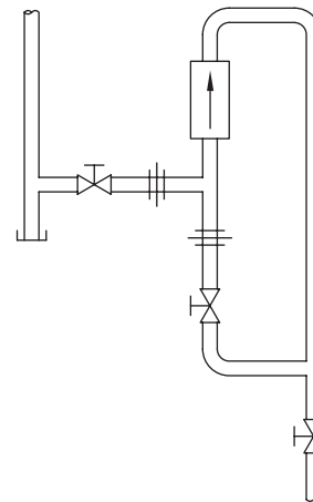
Figure CG-55-2. Typical Disc Trap Hookup
