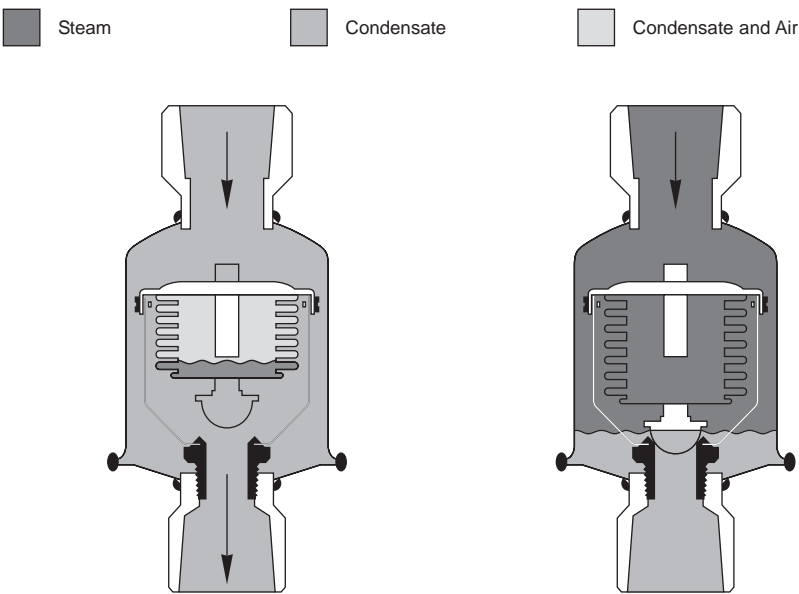
Figure CG-20-1. Operation of Thermostatic Steam Trap
