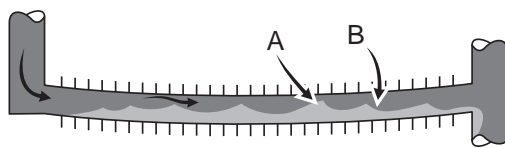
Figure CG-13-2. Condensate allowed to collect in pipes or tubes is blown into waves by steam passing over it until it blocks steam flow at point A. Condensate in area B causes a pressure differential that allows steam pressure to push the slug of condensate along like a battering ram.
