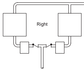
Figure CG-22-2. Short circuiting is impossible when each unit is drained by its own trap. Higher efficiency is assured.
