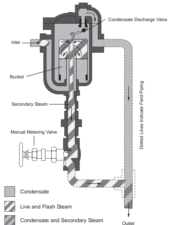
Figure CG-21-2. Condensate Controller Operation
