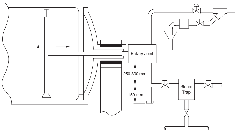
Figure CG-46-1. Product Outside Dryer
