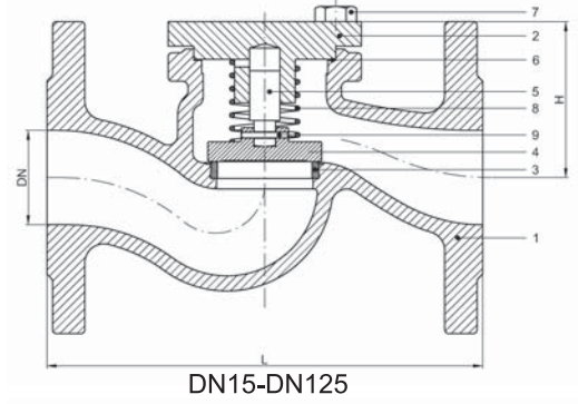
DN15-DN125
